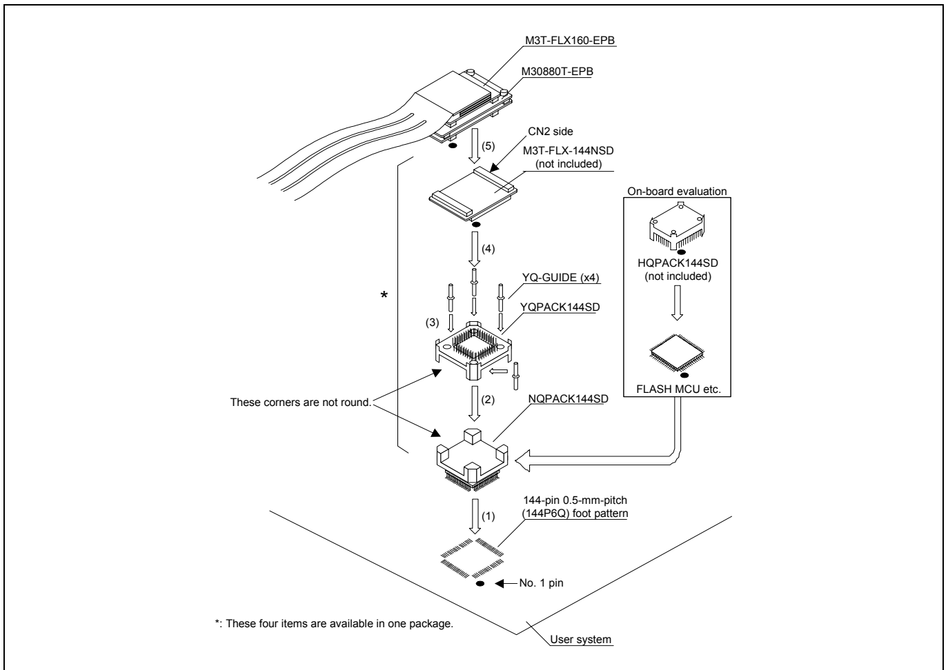
Figure 2.15 Connecting to a 144-pin 0.5-mm-pitch foot pattern
